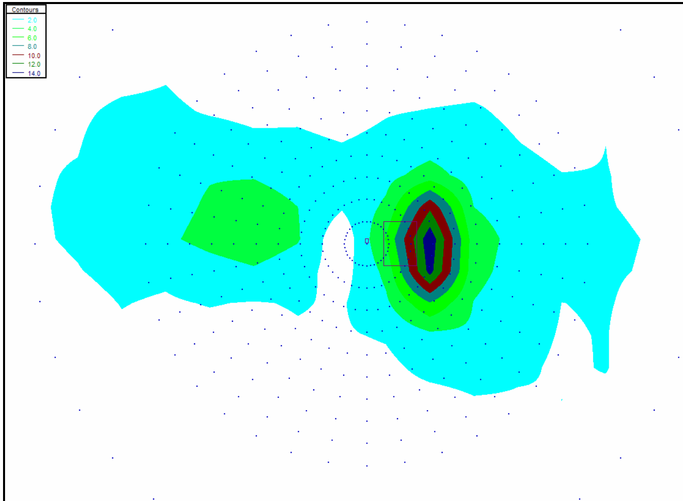
Figure 1. Maximum 8 th High PM 2.5 24-Hour Impact (22' Stack, 0.60 lb/MMBtu)
